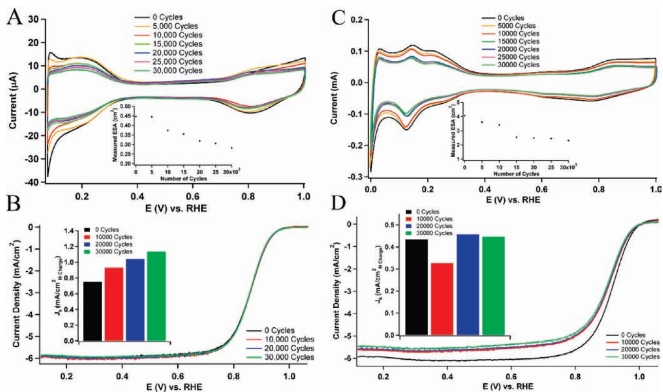
Figure 7. Cyclic voltammograms obtained in deoxygenated 0.1 M HClO 4 solution after 5000 cycles for the Pt–Pd NW/C core shell composites (A) and commercial high performance (HP) Pt/C catalysts (C). The measured ESA loss is also shown as a function of durability cycling for the Pt–Pd NW/C composites and HP Pt/C catalysts as insets to A and C, respectively. The polarization curves (anodic sweep direction) obtained in an oxygen saturated 0.1 M HClO 4 solution at 1600 rpm after 10 000 cycles for the Pt–Pd NW/C composites (B) and the HP Pt/C catalysts (D) are presented. Measured area-specific kinetic currents (ECSA) are also shown as a function of durability cycling for the Pt–Pd NW/C composites and the HP Pt/C catalysts as insets to B and D, respectively.
